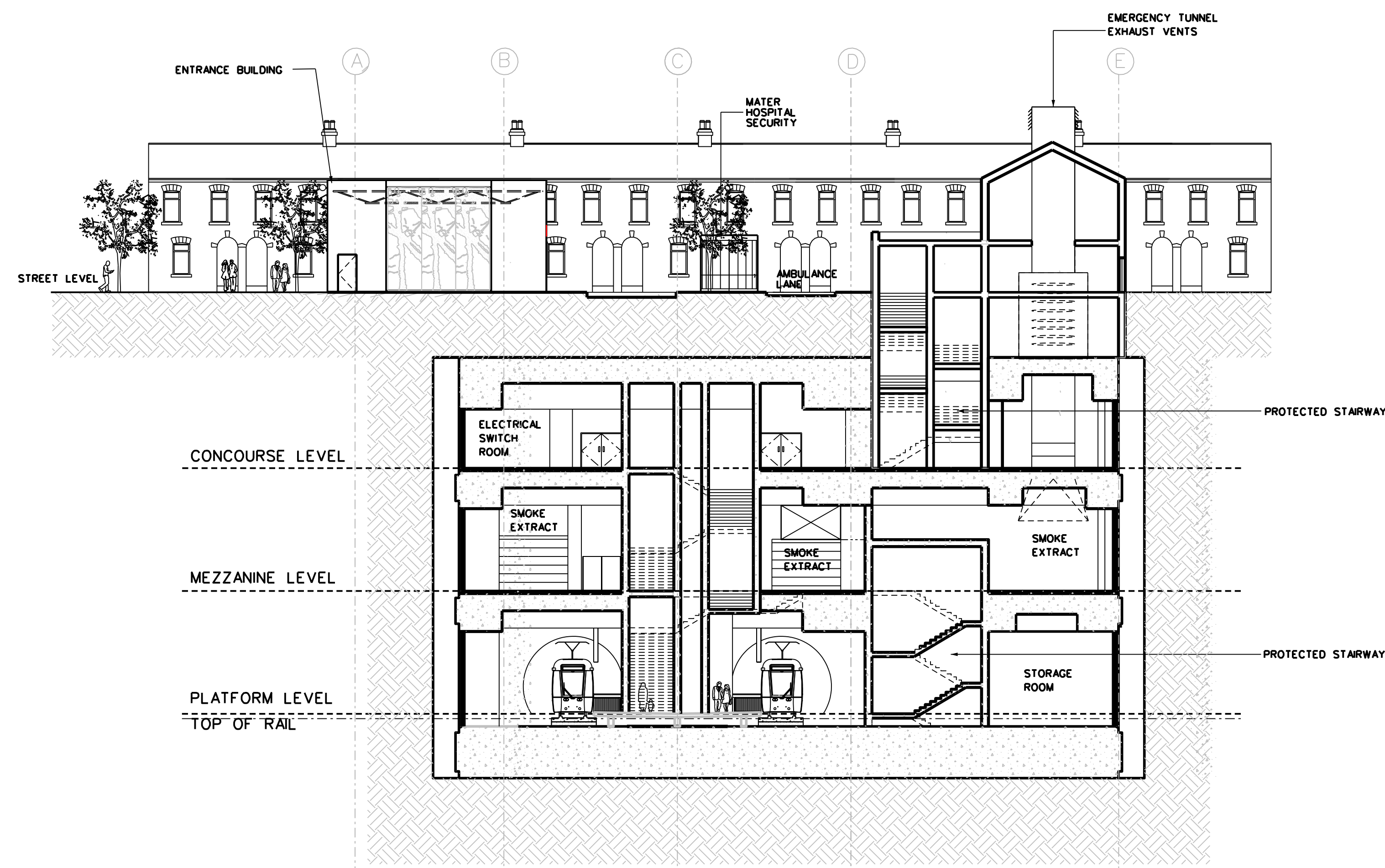
SECTION B-B SCALE 1:200
