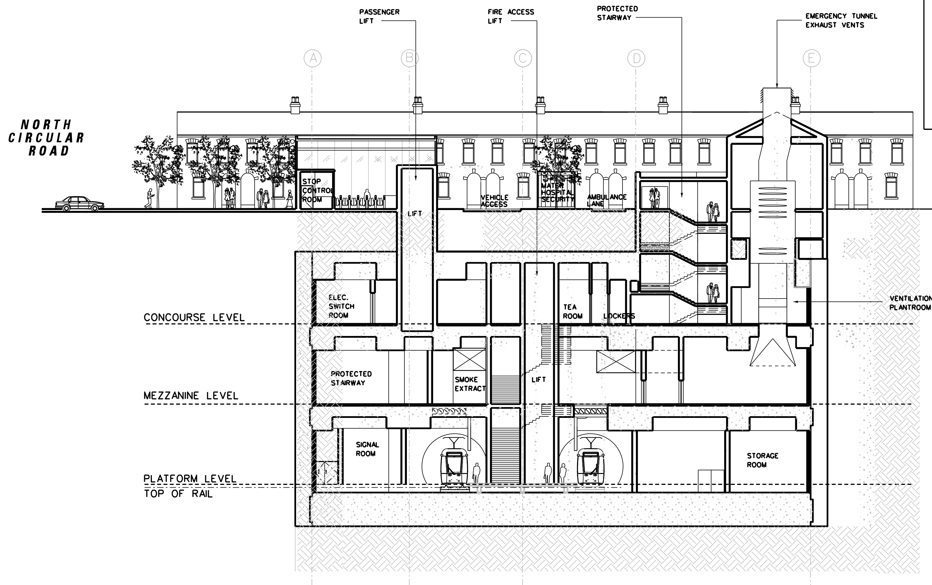
SECTION C-C SCALE 1:200
