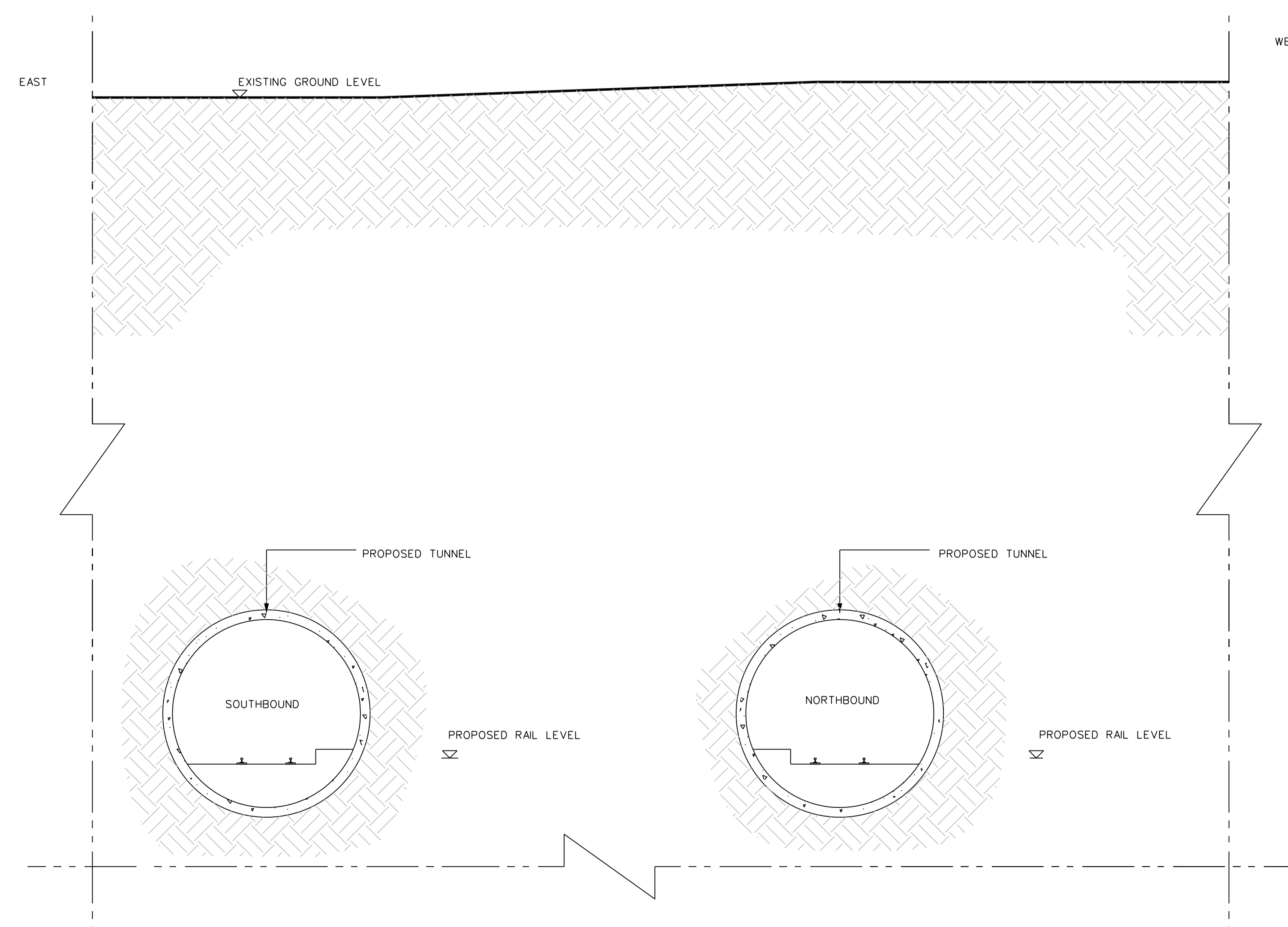
CROSS SECTION 03-05 SCALE 1:100
