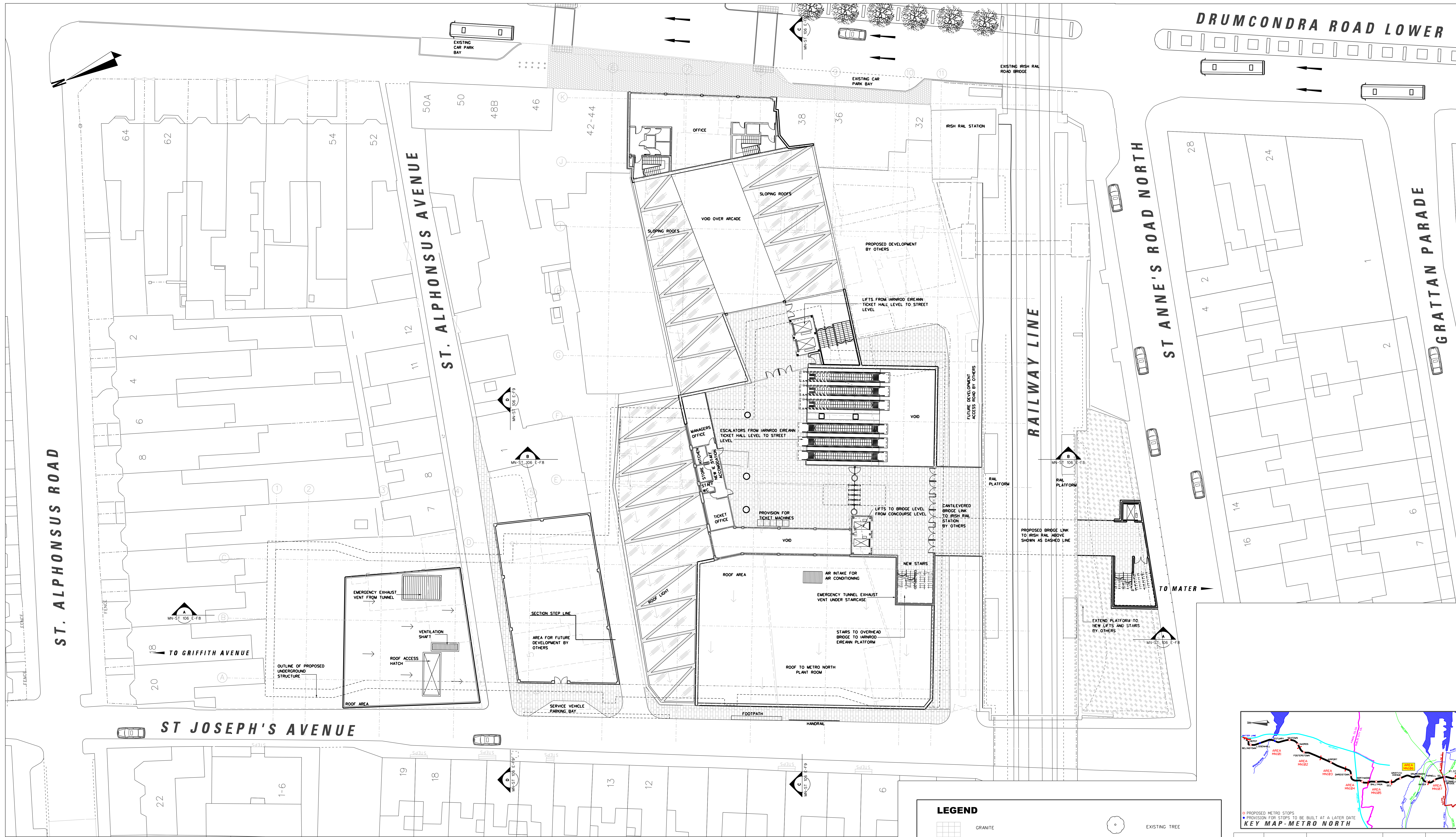
IARNROD EIREANN TICKET HALL LEVEL PLAN SCALE 1:200
