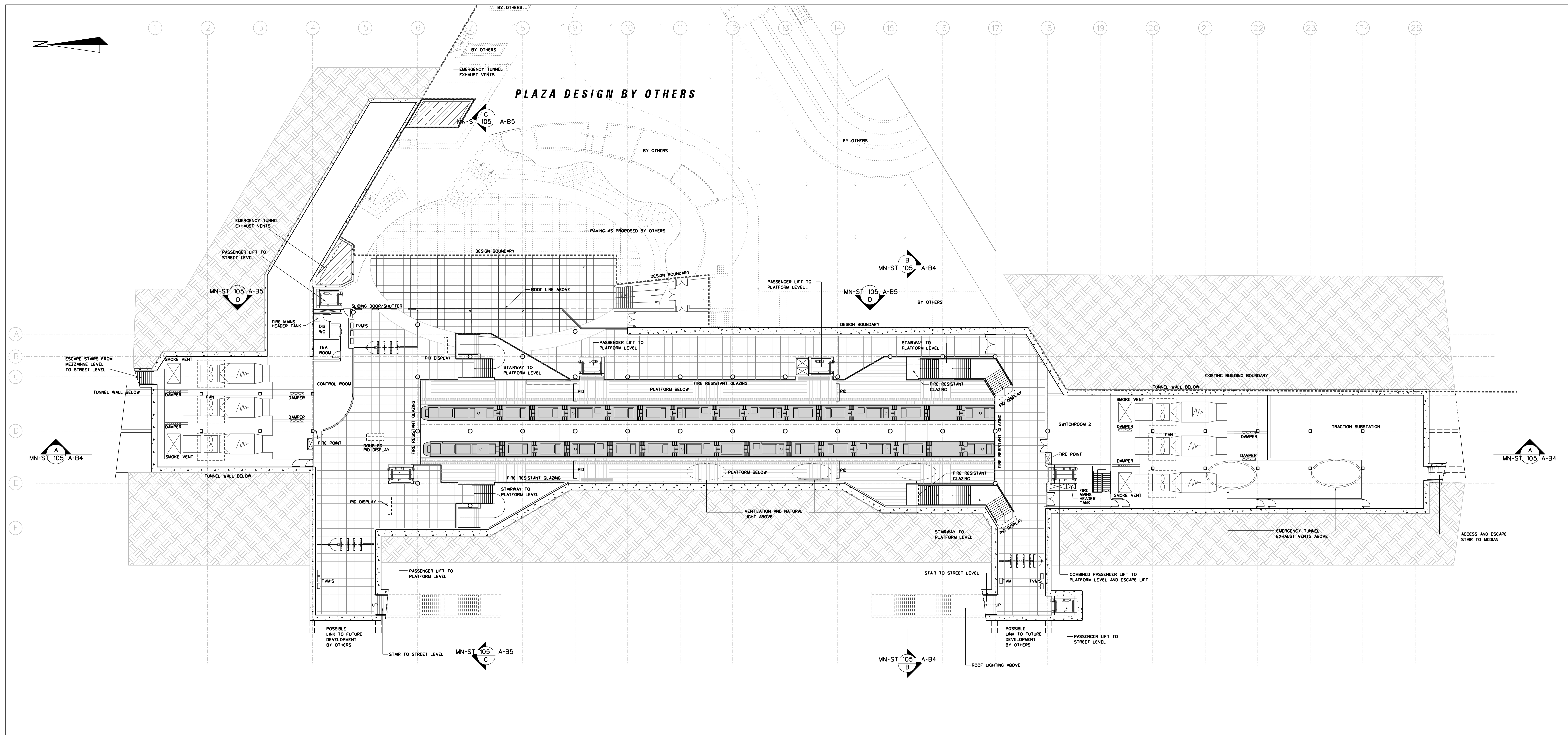
MEZZANINE LEVEL PLAN SCALE 1:200
