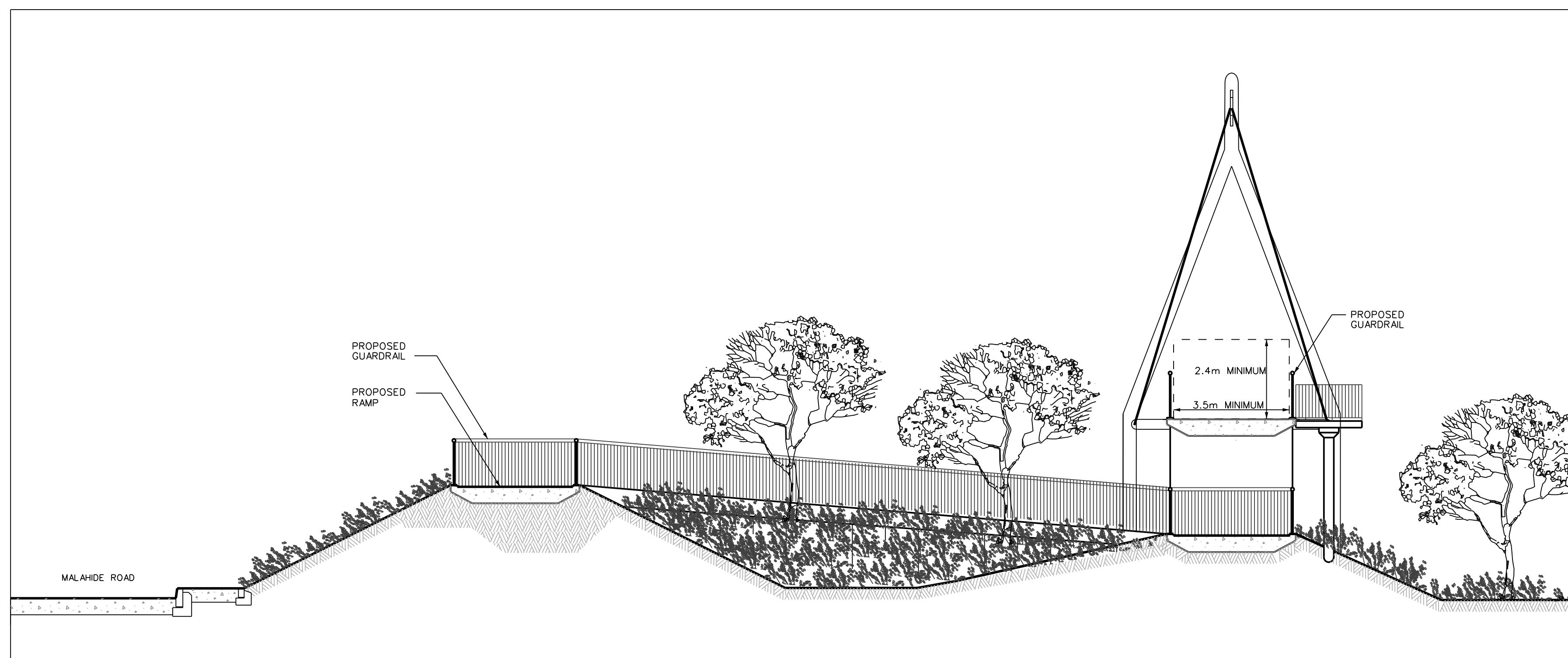
SECTIONAL ELEVATION B-B SCALE 1:100
