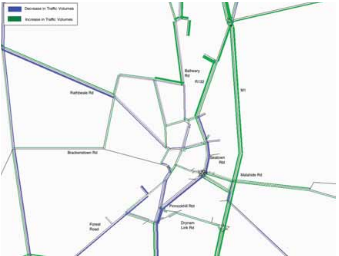
Figure 7.8 Traffic flow changes – do-minimum vs. do-something 2014 (Swords area)
