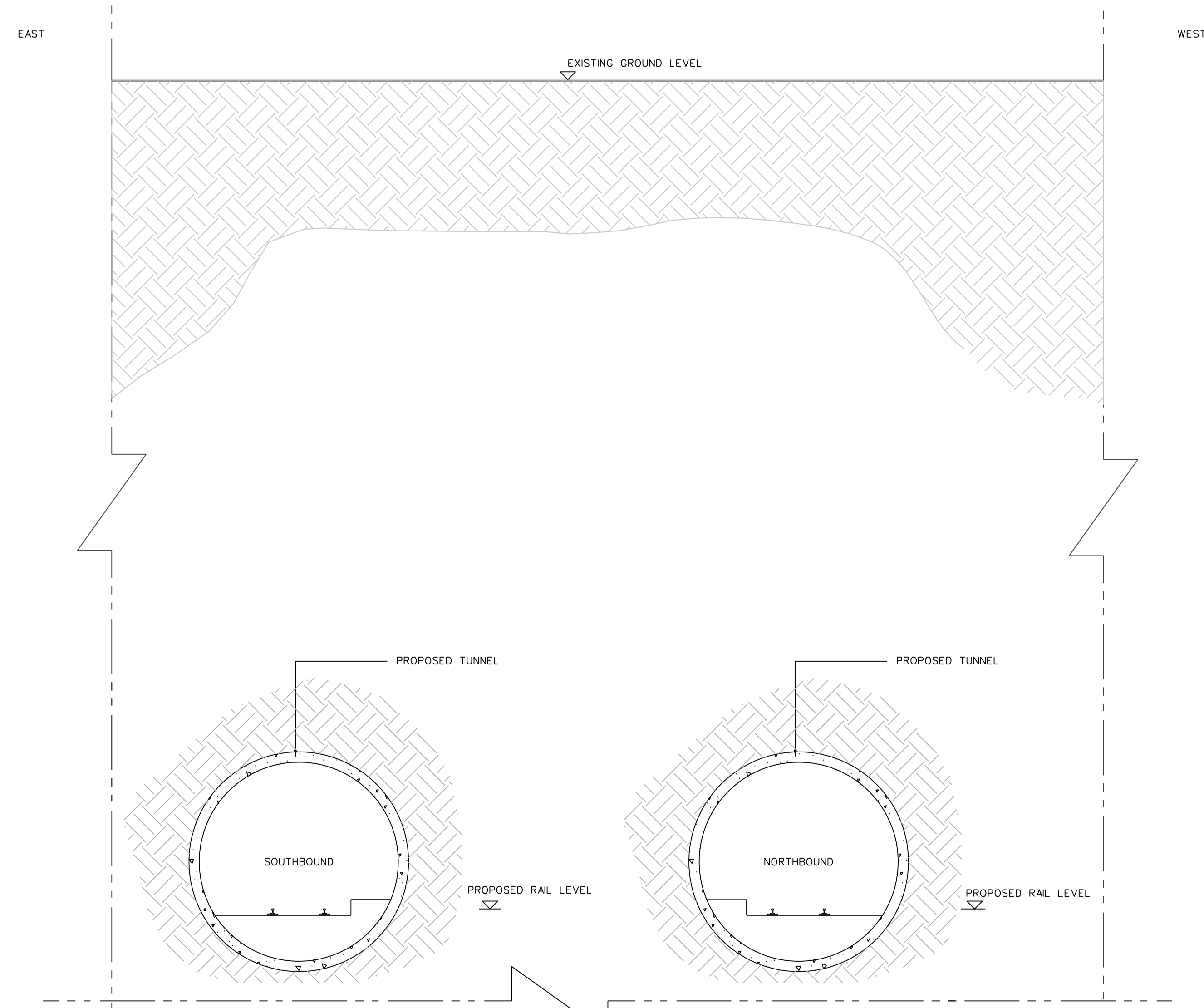
CROSS SECTION 06-07 SCALE 1:100
