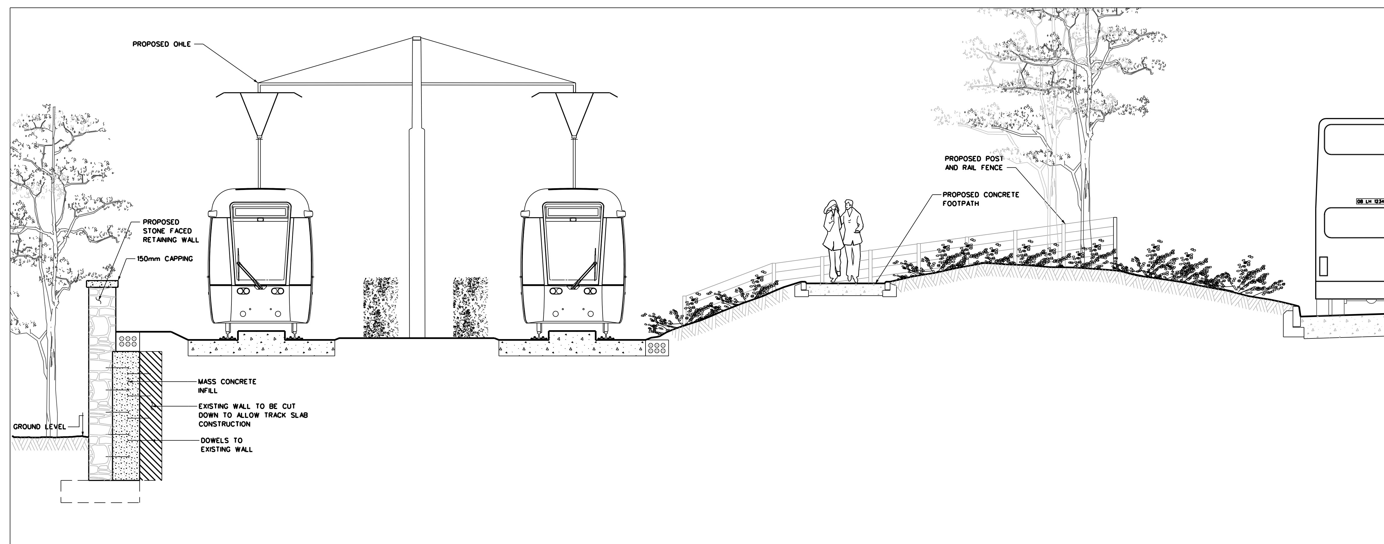
SECTION B-B SCALE 1:50
